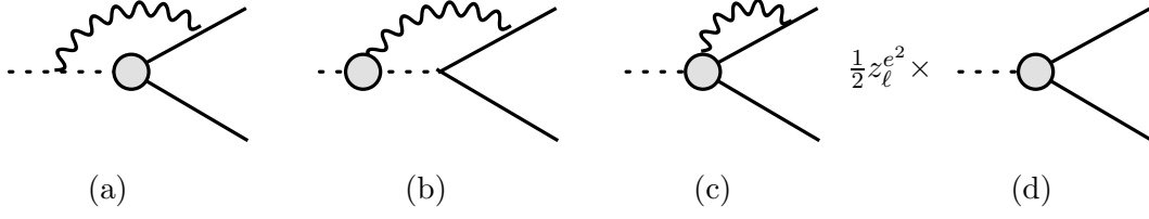
Figure 4: Effective one-loop diagrams contributing to R_{e/\mu} to order e^2 p^4 . The shaded circles represent the O(p^4) contribution to d-dimensional off-shell effective vertices.
