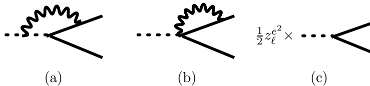
Figure 1: Diagrams contributing to R_{e/\mu} to order e^2 p^2 . Dashed lines indicate pseudoscalar mesons, solid lines leptons, and wavy lines photons.
