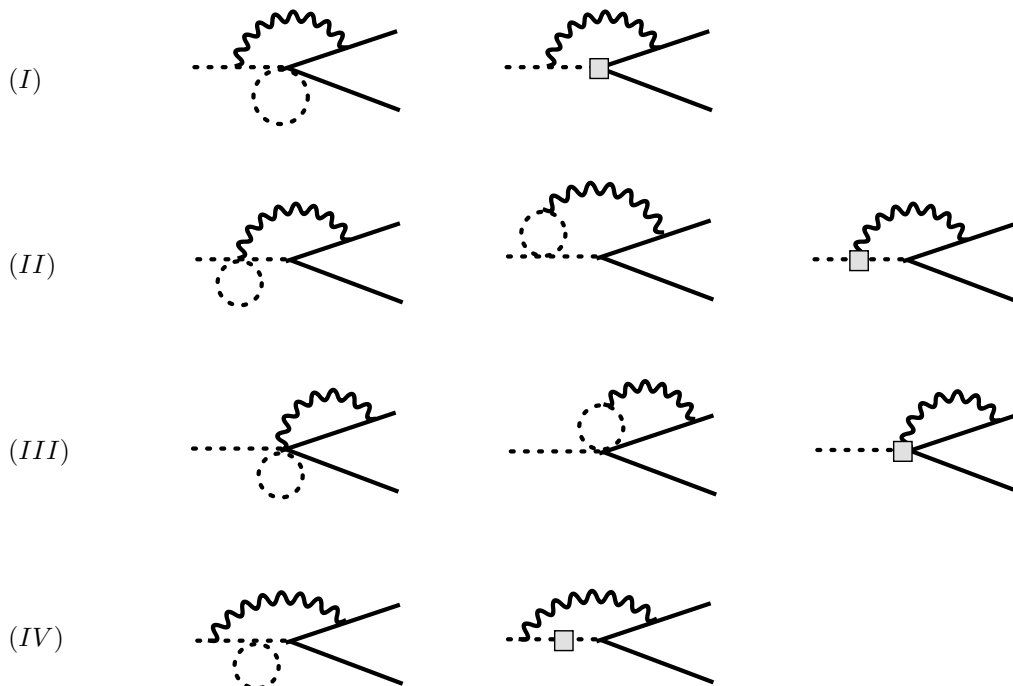
Figure 2: 1PI diagrams contributing to R_{e/\mu} to order e^2 p^4 . Shaded squares indicate vertices from the O(p^4) effective lagrangian.
